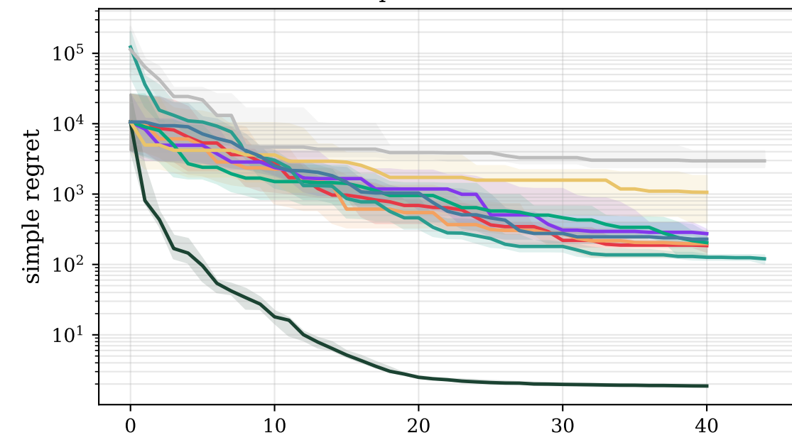
SpeedReducer
